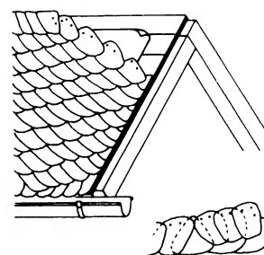
12 German slate roof, 0.45-0.6 kN/m 2
